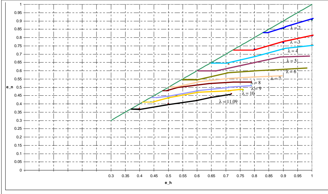
Figure 1: Admissible values for the domestic and the new technology parameters e_h and e_n respectively, for different values of the environmental damage parameter \lambda .
