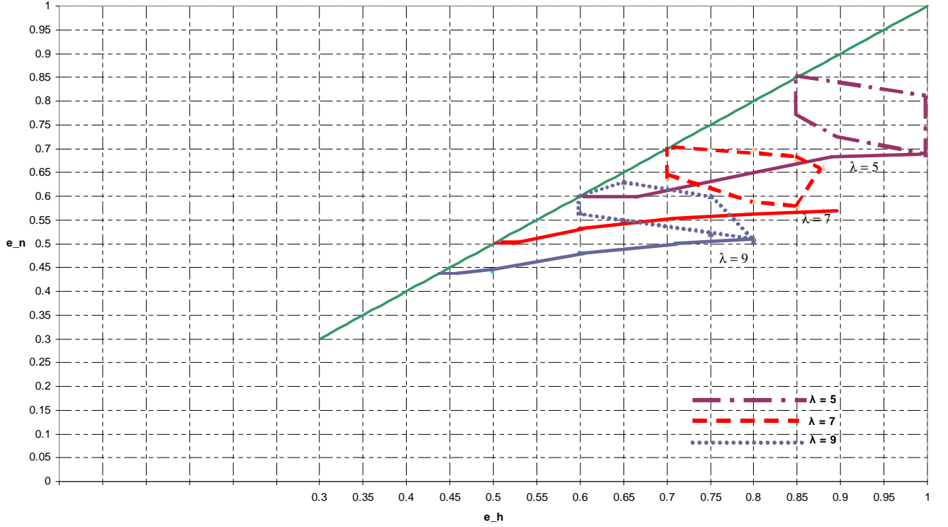
Figure 4: Values of e_h , e_n and \lambda for which (50) does not hold when e_f is close to e_n
