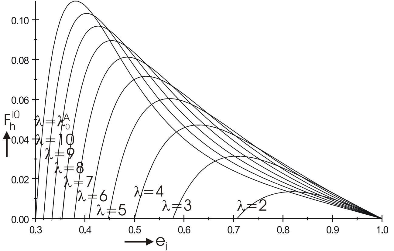
Figure 2: The domestic firm's licence fee F_h^{i0} under autarky when the domestic firm has technology e_i , i = h, n .
