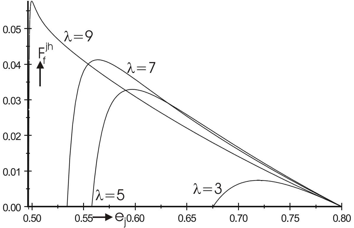
Figure 3: The foreign firm's licence fee F_f^{jh} when the foreign firm has technology e_j , j = f, n , and the domestic firm has technology e_h = 0.8 .
