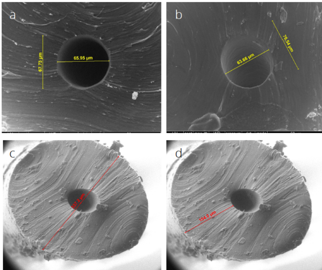
Figure 3. SEM images of the lumen diameter measured with the caliper tool. (a) Luminal diameter 67.73 × 65.95 μm. (b) Luminal diameter 63.66 × 70.54 μm. (c) Total diameter: 337.2 μm. (d) Wall: 154 μm.
