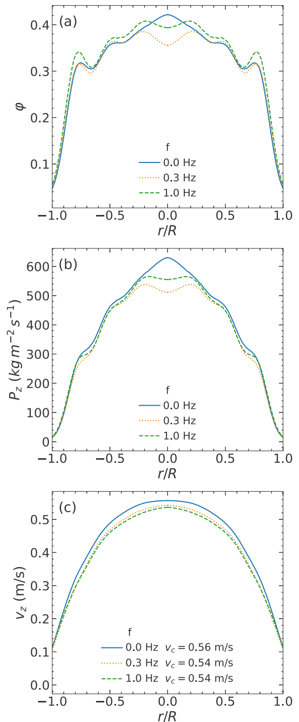
FIG. 9. Spatial profiles at the orifice ( z = 0 ) for D = 36 mm ( 6.20 D/d ) in (a) average density field \langle \phi(r) \rangle , (b) average momentum on the vertical direction \langle P_z(r) \rangle , and (c) average velocity on the vertical direction \langle V_z(r) \rangle . In each case, finding corresponding to rotational frequency [ f = 0; 0.3; 1.0 ] in Hz are shown.
