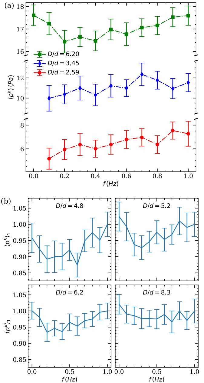
FIG. 11. Mean kinetic pressure \langle p^k \rangle = \text{Tr}(\langle \sigma^k \rangle_{ts}) , averaged in the region of the orifice as a function of the rotation frequency f . (a) Data obtained for D = 15 \text{ mm} , D = 20 \text{ mm} , and D = 36 \text{ mm} . (b) Data \langle p^k \rangle_1 = \langle p^k \rangle / \langle p^k \rangle_{f=1 \text{ Hz}} normalized by its value at f = 1 \text{ Hz} for D = 28 \text{ mm} , D = 30 \text{ mm} , D = 36 \text{ mm} , and D = 48 \text{ mm} . In each case, the error bars represent confidence intervals for the mean with 95% of confidence level.
